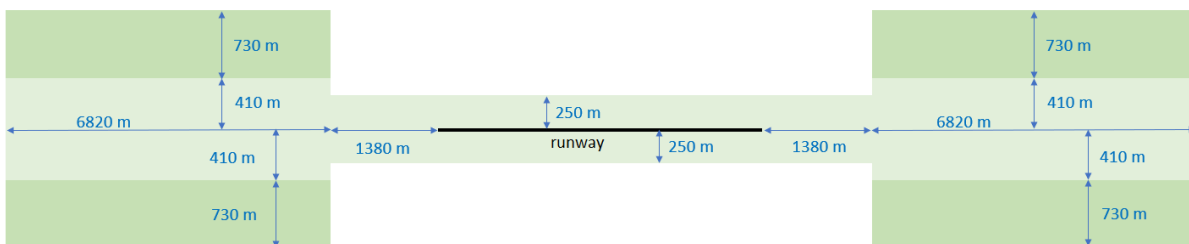
Figure 4: Example zone sizes definitions – where only one approach to a runway requires protection (not to scale)
