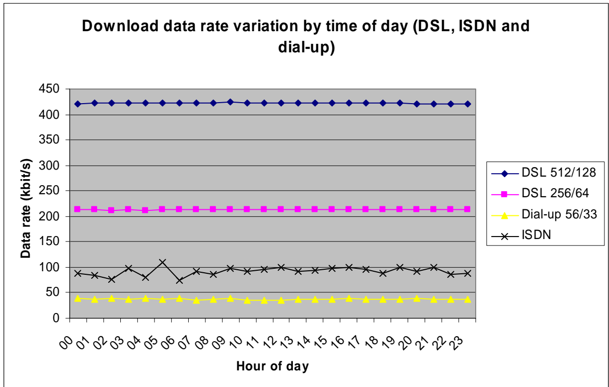
Figure B.2: Average download data rates (kbit/s) for each hour of the day (DSL, ISDN, dial-up)
