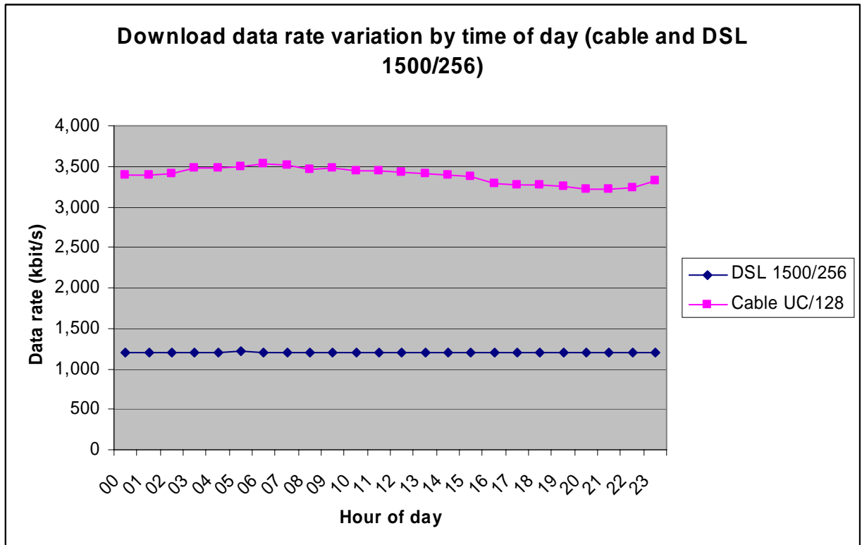
Figure B.1: Average download data rates (kbit/s) for each hour of the day (cable and DSL 1500/256)
